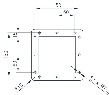
BACKING FLANGE
