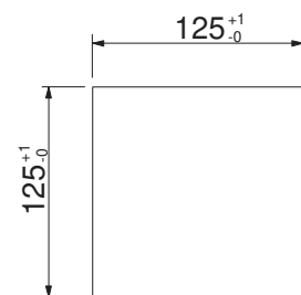
Cut-Out Dimensions
