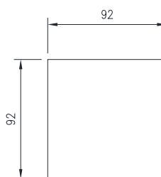
CUT-OUT DIMENSION
