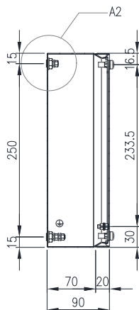
SECTION B-B
