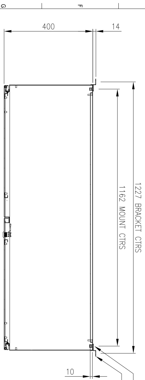
SECTION AW-AW
