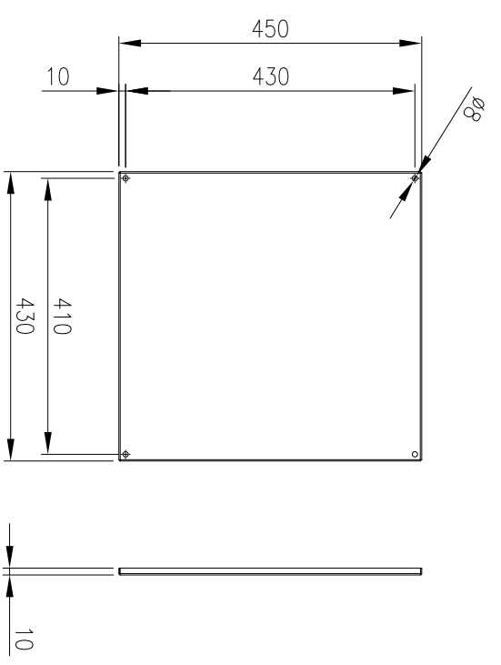
INSIDE DOOR VIEW
