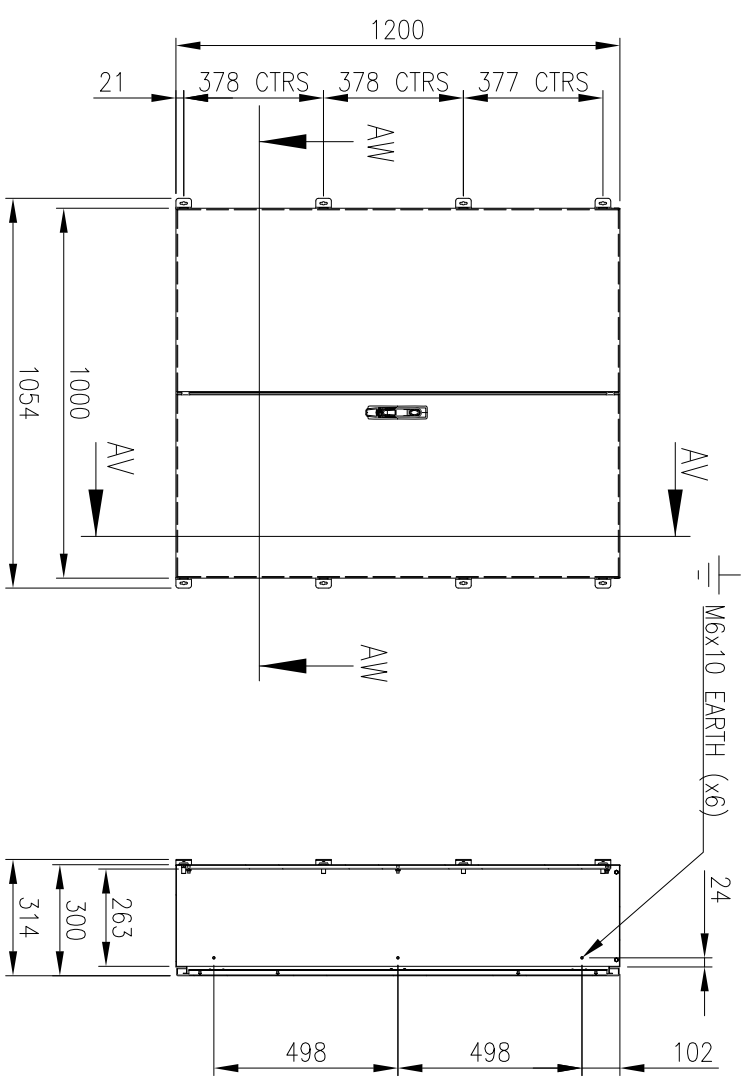
FRONT VIEW
