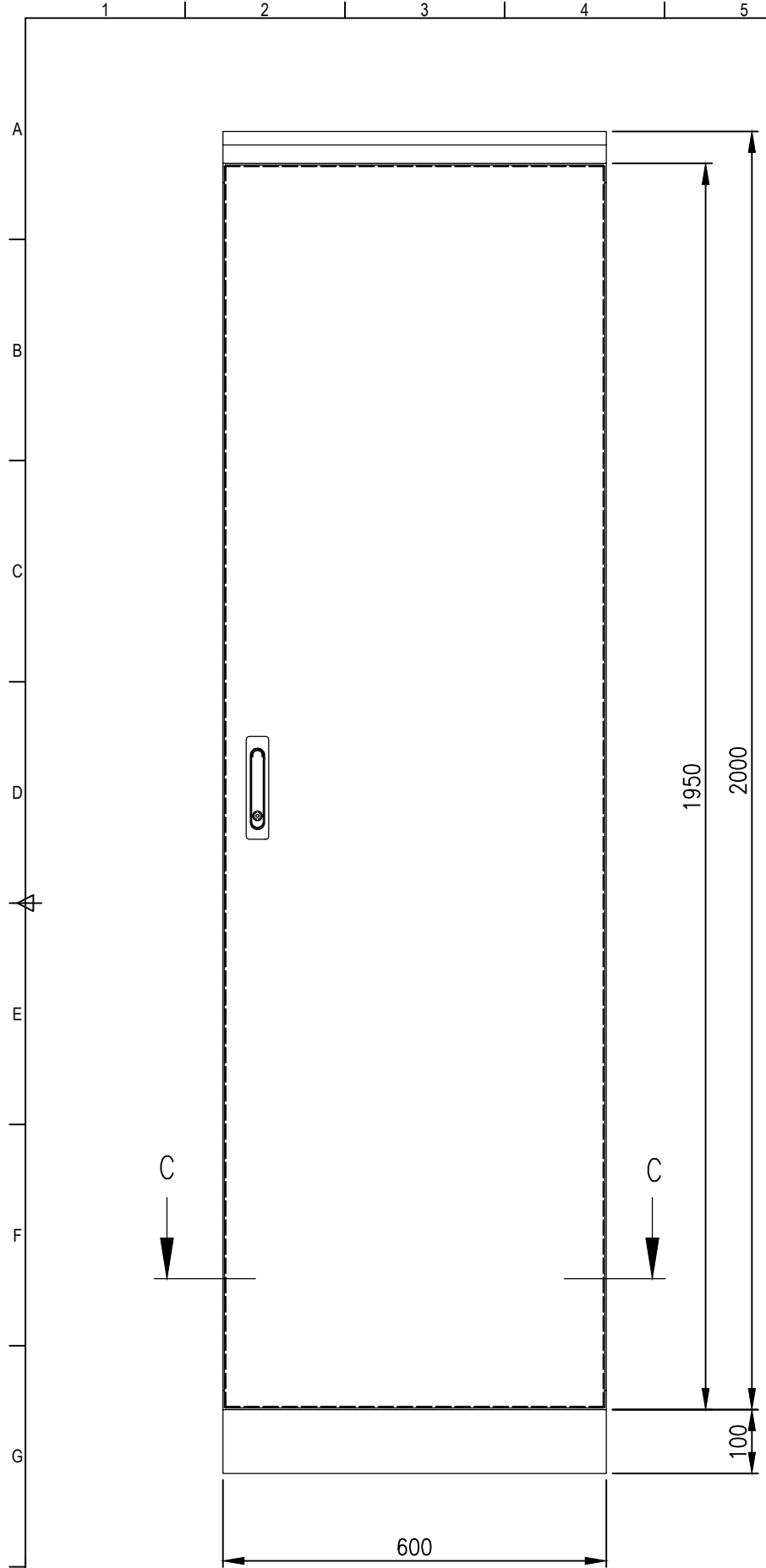
FRONT VIEW
