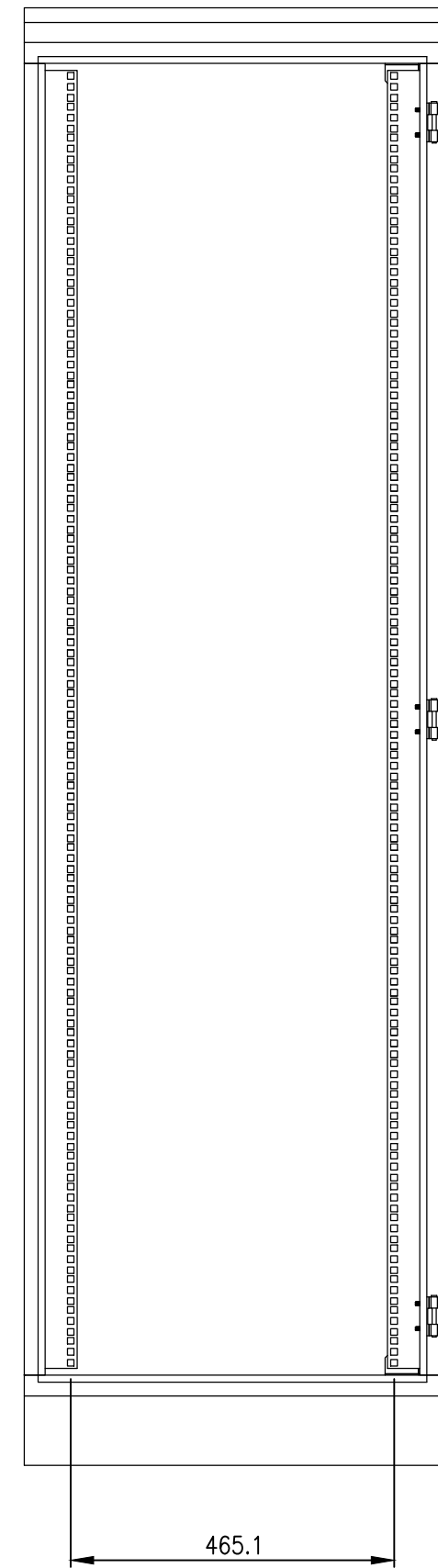
SECTION AA
