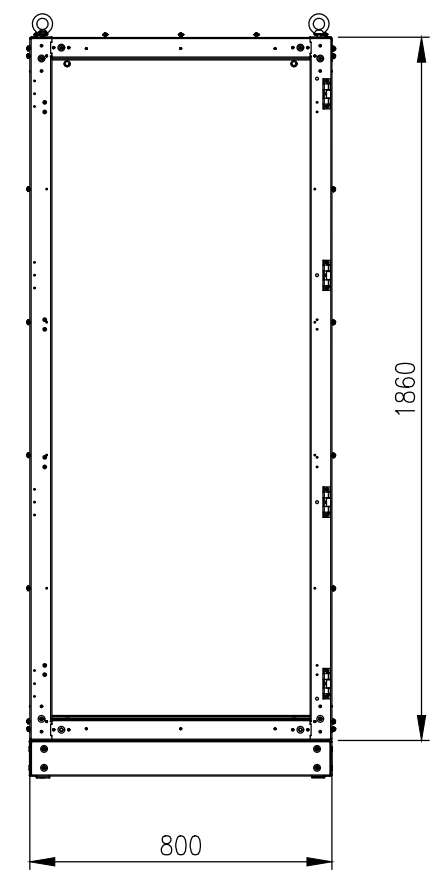
FRONT VIEW (PANELS REMOVED)
