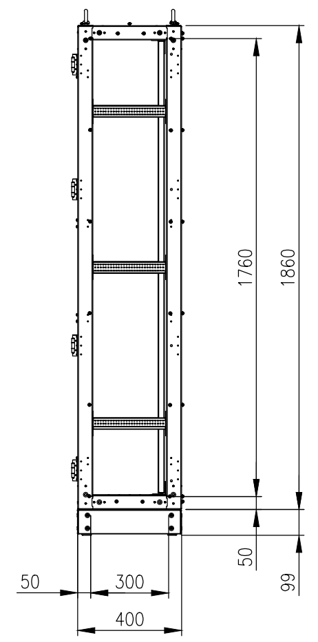
SIDE VIEW (PANELS REMOVED)
