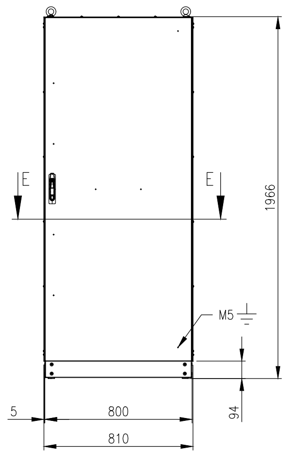
FRONT VIEW (ASSEMBLY)
