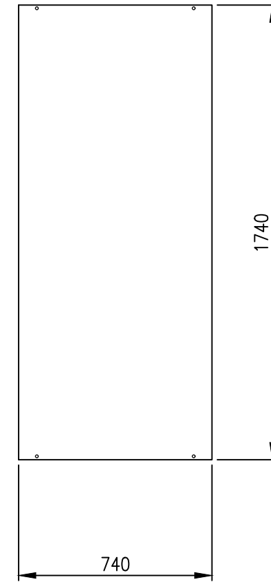
DEVICE MOUNTING PLATE
