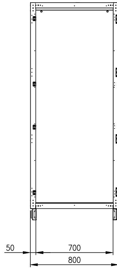
FRONT VIEW (PANELS REMOVED)
