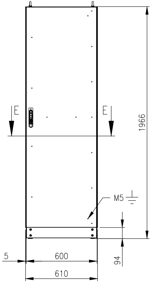
FRONT VIEW (ASSEMBLY)
