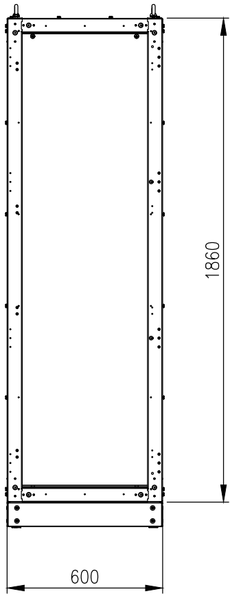
FRONT VIEW (PANELS REMOVED)
