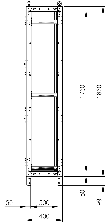
SIDE VIEW (PANELS REMOVED)
