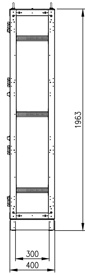
SIDE VIEW (PANELS REMOVED)
