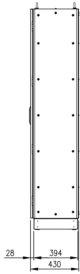
SIDE VIEW
