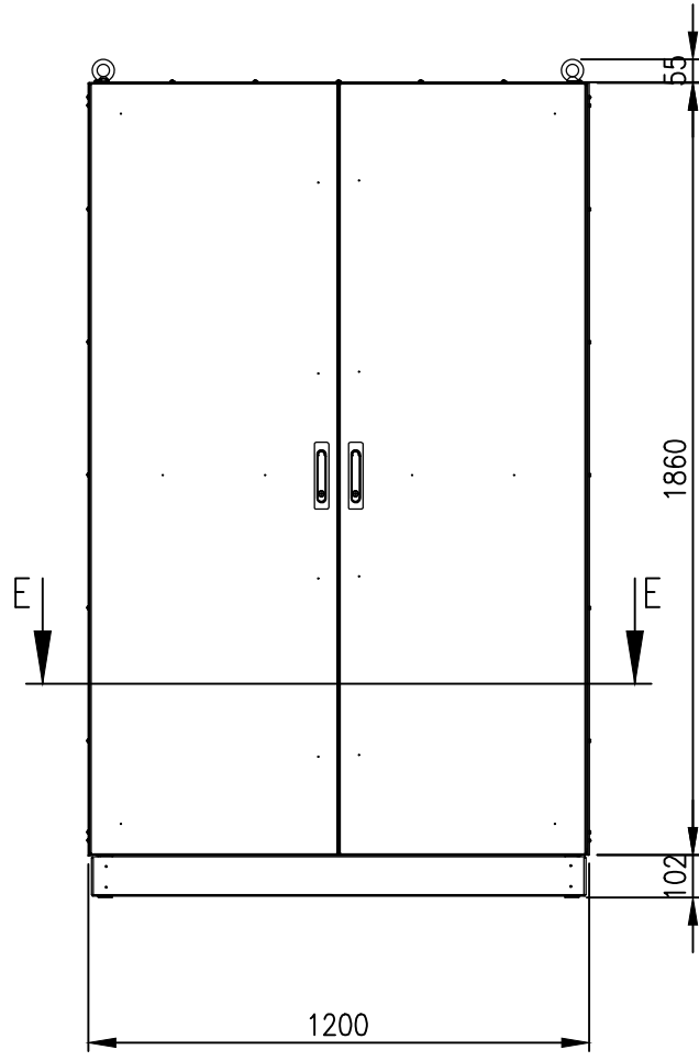
FRONT VIEW (ASSEMBLY)
