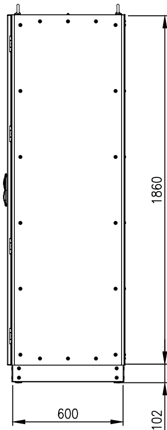
SIDE VIEW
