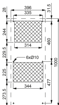
MOUNTING CUT-OUT
