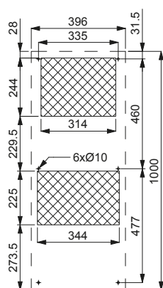
MOUNTING CUT-OUT
