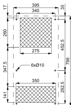
MOUNTING CUT-OUT
