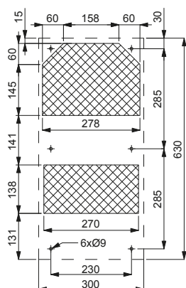
MOUNTING CUT-OUT
