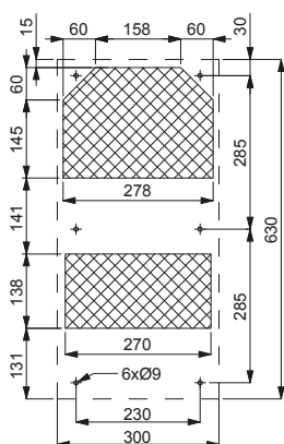
MOUNTING CUT-OUT
