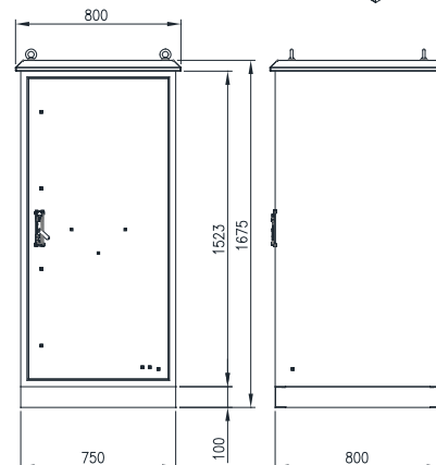
FRONT VIEW (ASSEMBLY)
