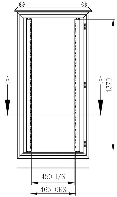
FRONT VIEW (FRONT DOOR REMOVED)
