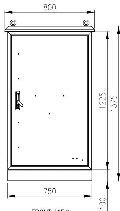
FRONT VIEW (ASSEMBLY)
