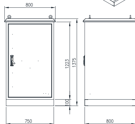
FRONT VIEW (ASSEMBLY)
