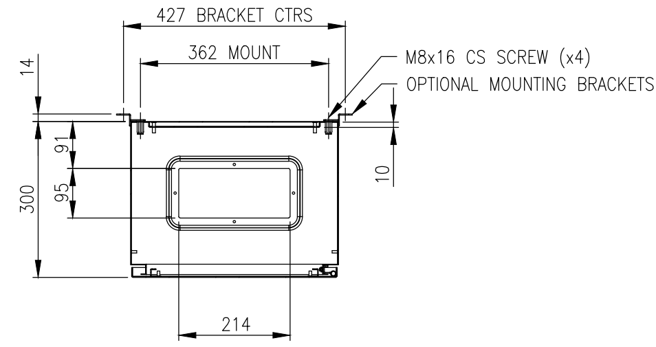
SECTION AW-AW
