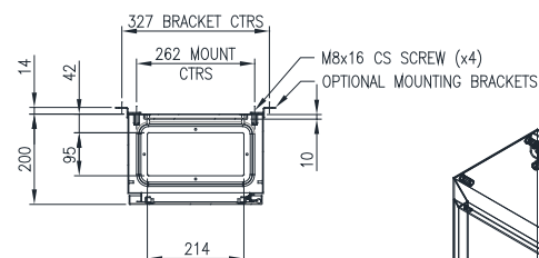
SECTION AW-AW
