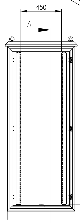
FRONT INTERIOR VIEW (DOOR REMOVED)
