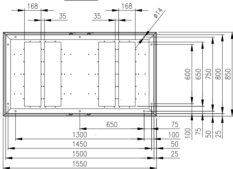
BOTTOM VIEW
