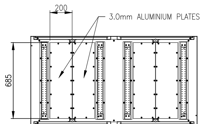
INTERIOR VIEW-DOOR REMOVED
