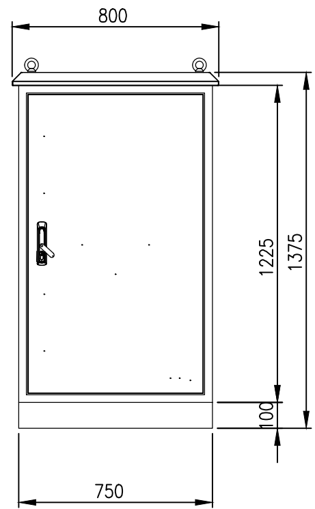
FRONT VIEW (ASSEMBLY)
