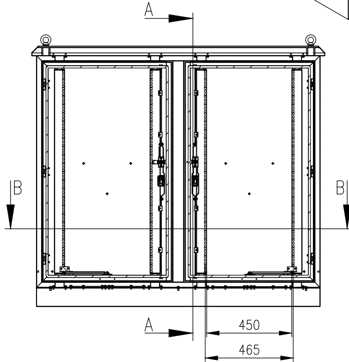
FRONT VIEW—DOOR REMOVED
