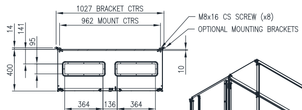
SECTION AW-AW
