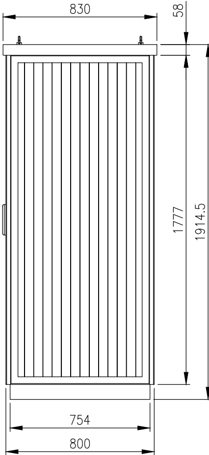
SIDE VIEW
