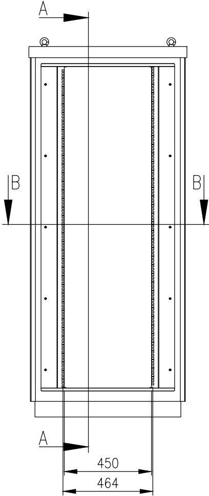
FRONT VIEW-DOOR REMOVED
