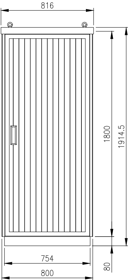
FRONT VIEW
