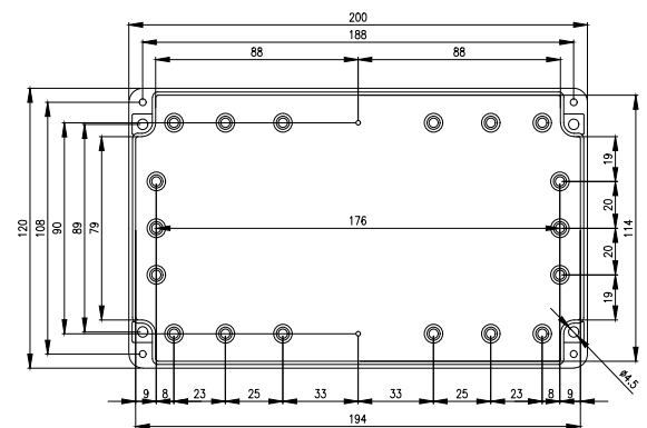
FRONT VIEW-DOOR REMOVED
